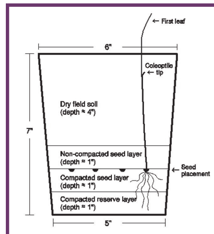
Figure 1. Cross-section illustration of a prepared pot for measuring wheat seedling emergence in the laboratory. Four distinct soil layers as required: a) compacted reserve layer; b) compacted seed layer; c) non-compacted layer on top of the seed; and d) thick layer of loose, dry soil that extends to the top of the pot.
