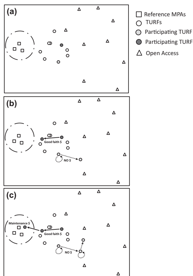
Figure 3. Multidimensional scaling plot that represents subtidal community assemblages associated with no-take marine protected areas (MPAs), territorial user rights for fisheries (TURFs), and de facto open access areas under (a) current conditions and under 2 hypothetical periods after implementation of a crediting scheme: (b) after the first monitoring period and (c) after a series of monitoring periods. The current condition is for 38 reef fish and invertebrate species associated with 100-m transects reported in Gelcich et al. (2012). On all graphs, the dotted circle is the multivariate space used to define credits and black and gray dots are 2 TURFs in the crediting program. In (a) and (b) black dots show the TURF that comes close to the community structure of reference MPAs (solid line) and receives a good faith payment and gray dots show the TURF with no improvement in its trajectory (dotted line) that receives no payment (NO $). In (c) black dots show the TURF that becomes part of the multivariate space for receiving credits associated with an MPA and gray dots show the TURF that remains associated with the community structure of TURFs and does not improve, in which case they receive no payment.
