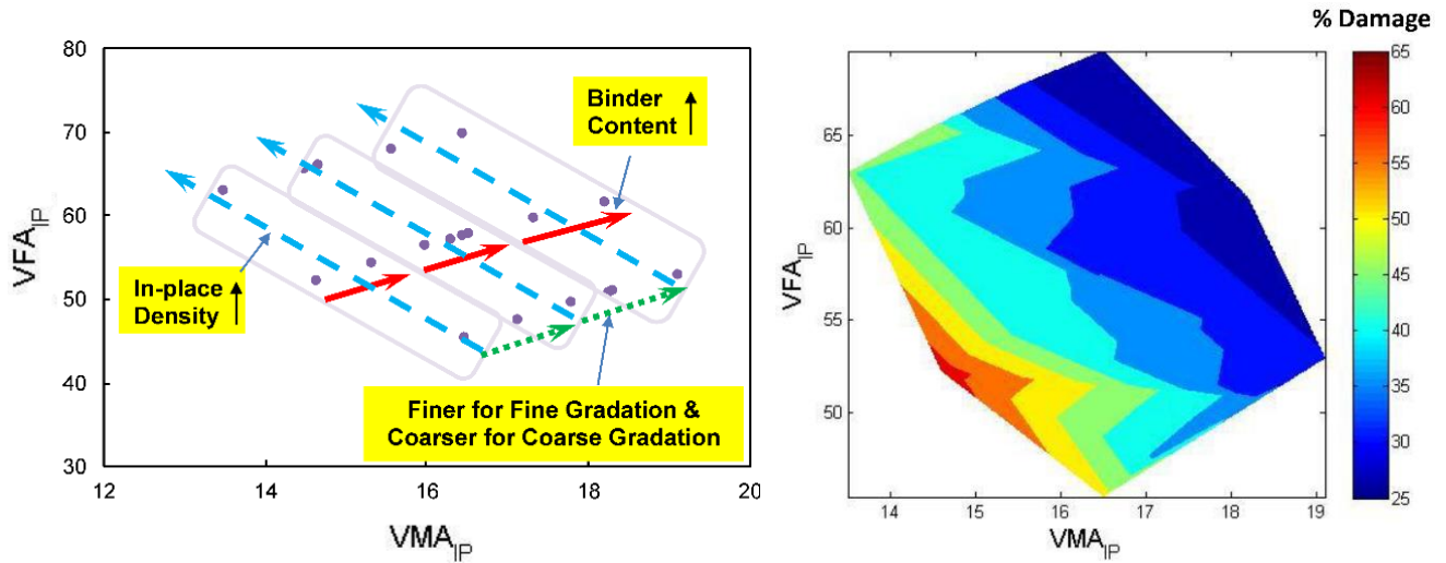
Figure 2.3 (a) Volumetric space formed by VMA IP and VFA IP and effects of mix design parameters on VMA IP and VFA IP and (b) %Damage contour in a pavement structure in the volumetric space (Wang et al. 2019)
