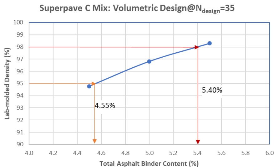
Figure 3.10 Volumetric Mix Design: Density vs. Asphalt Content
