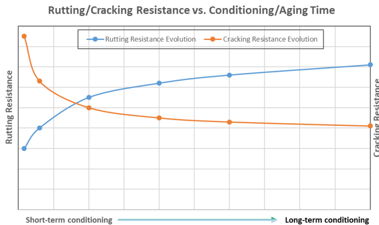
Figure 3.5 Rutting and Cracking Resistance Evolution vs. Conditioning/Aging Time
