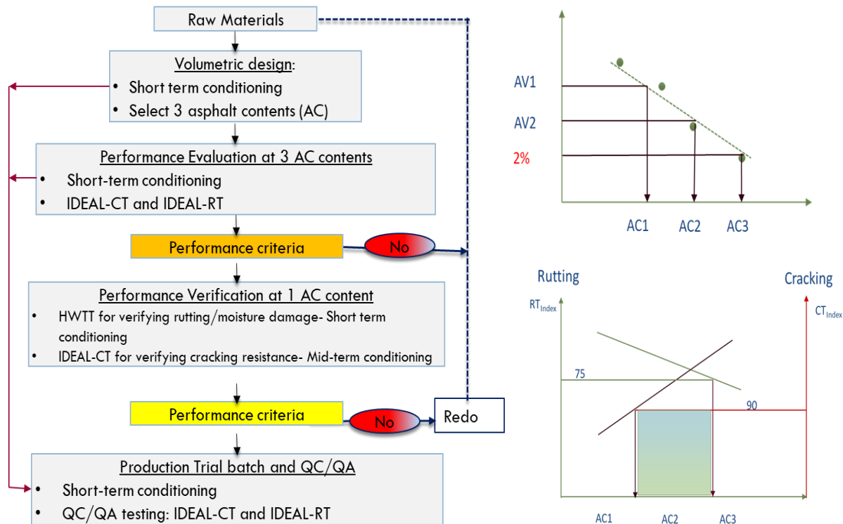
Figure 3.2 Coherent Framework for BMD/QC/QA: Example One with Index Tests
