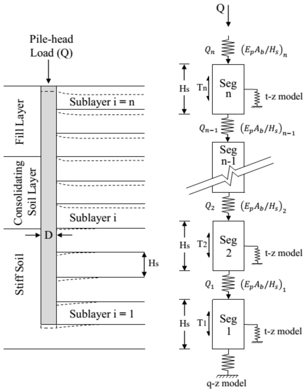
Fig. 5-7. Soil-pile modeling in sublayers and segments with a set of t-z and q-z springs.
