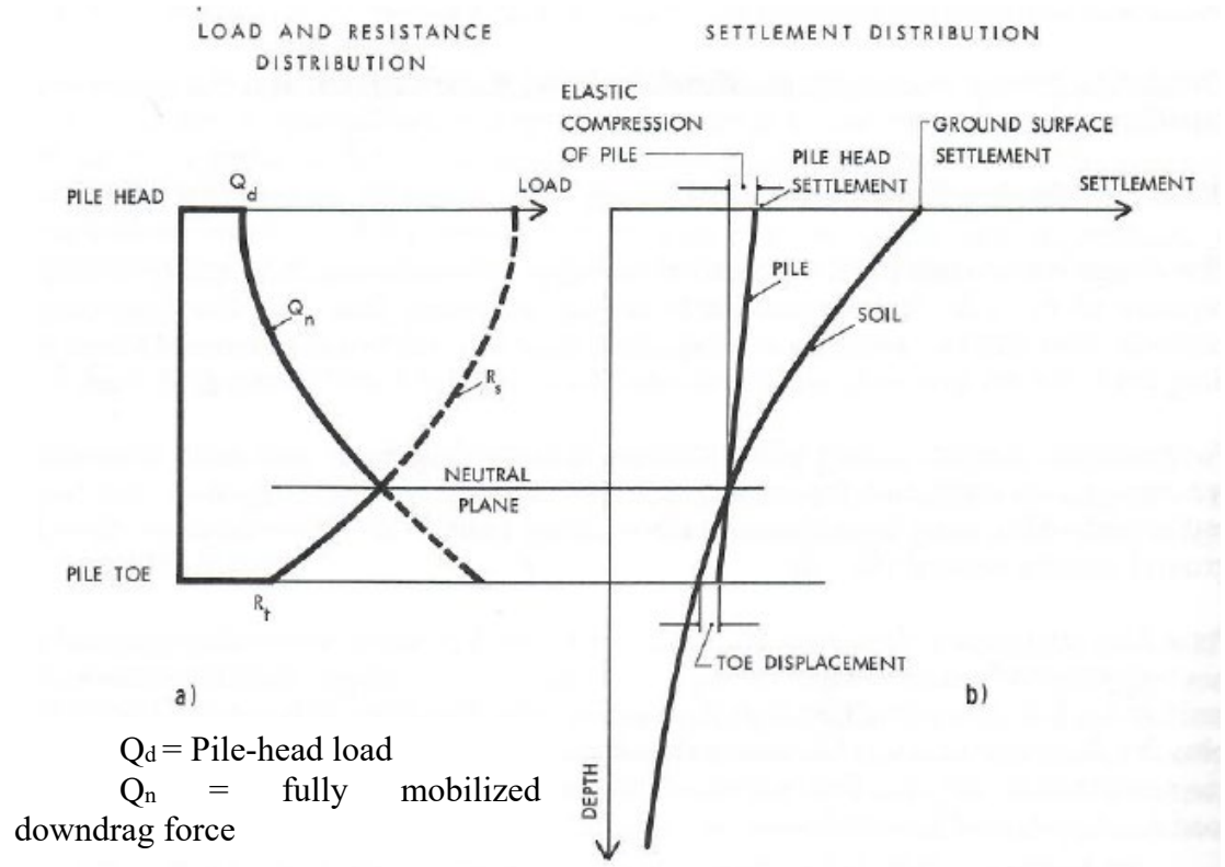
Fig. 1-3. FHWA/Pioneering work of Fellenius' method for the calculation of the downdrag force on piles induced by the soil consolidation settlement based on ultimate downdrag and pile resistance force distribution.
