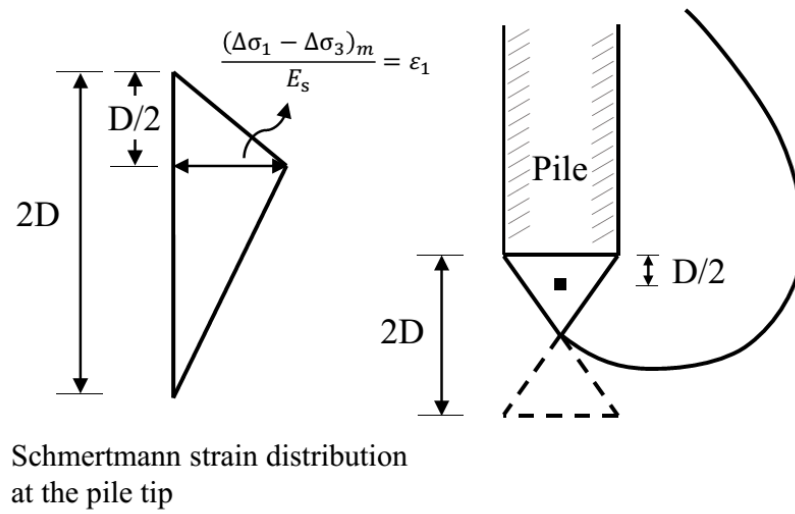
Fig. 3-7. Strain profile and the associated mobilized stresses immediately below the pile tip (after Elfass, 2001)
