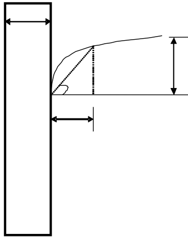
Fig. 4-3. Idealized relationship between shear strain in soil and pile displacement ( Norris 1986).
