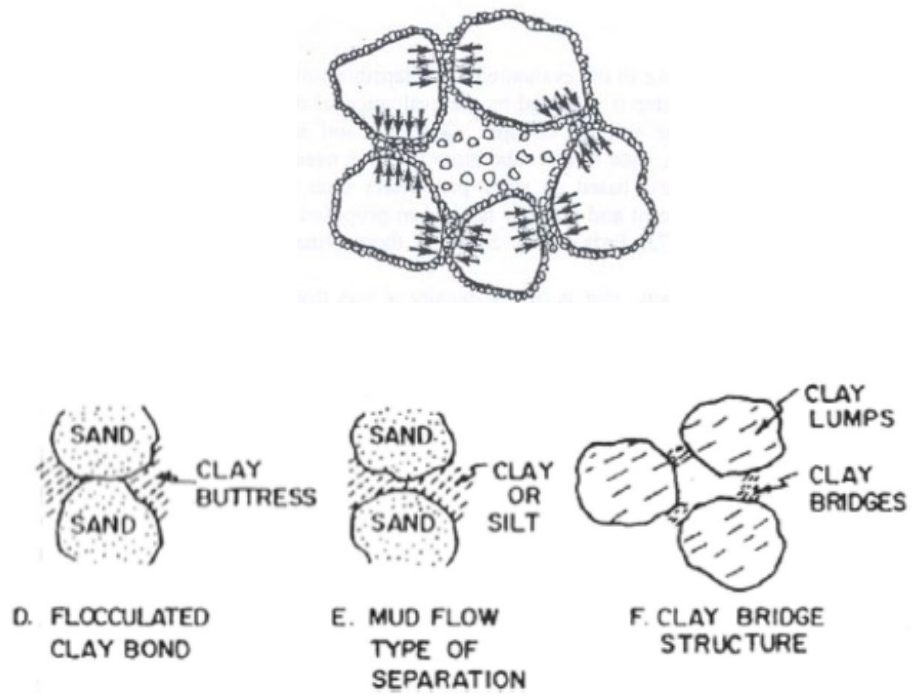
Fig. 2-1. Typical bonding structures of collapsible soils (Clemence and Finbarr 1981).
