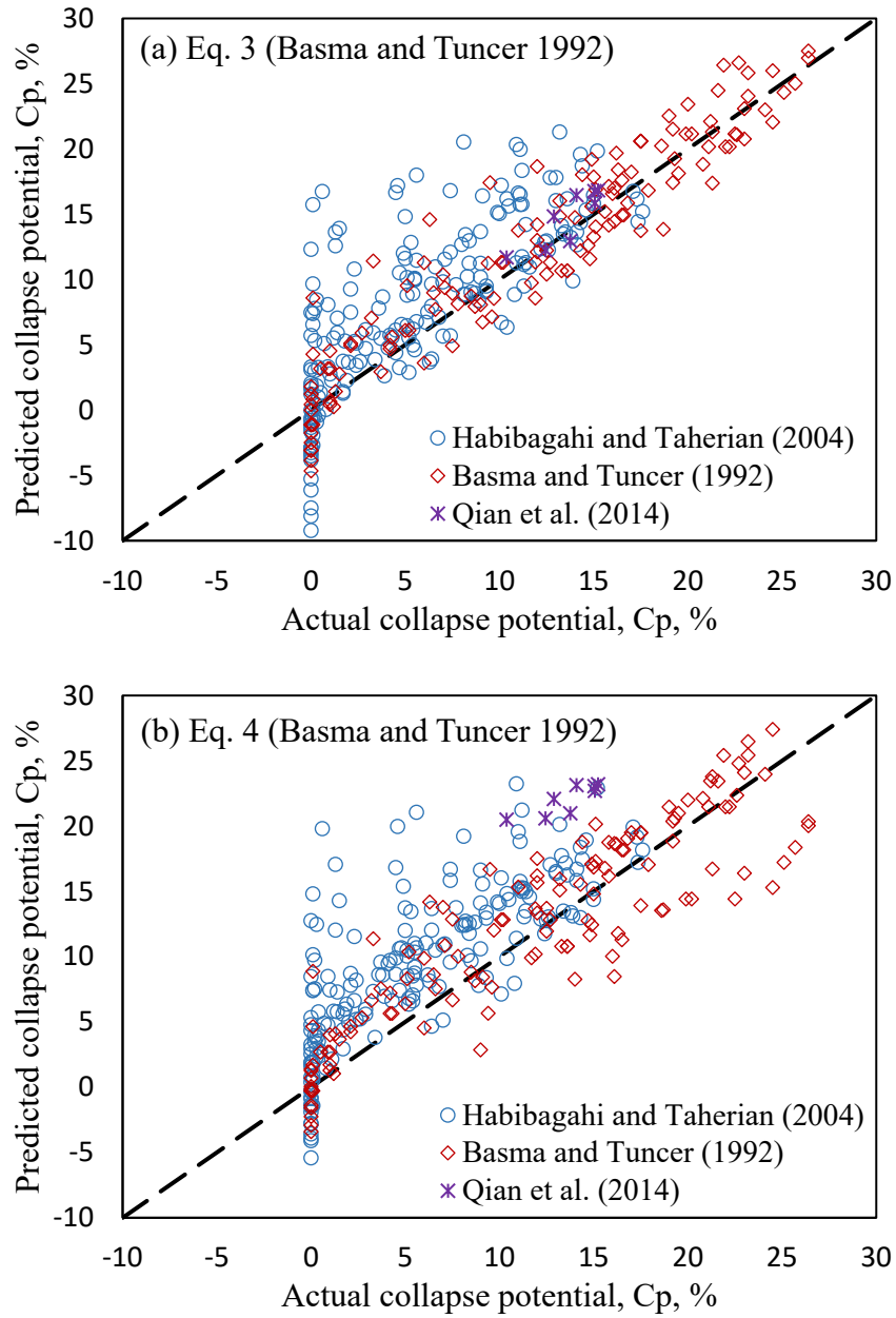
Fig. 2-7. Predictions of Eqs. 3 and 4 versus experimental data of inundated collapsible soils.
