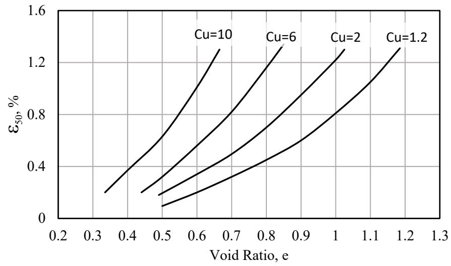
Fig. 2-10. Relationship between ( \epsilon_{50} ), uniformity coefficient ( C_u ) and void ratio ( e ) after Norris (1986)
