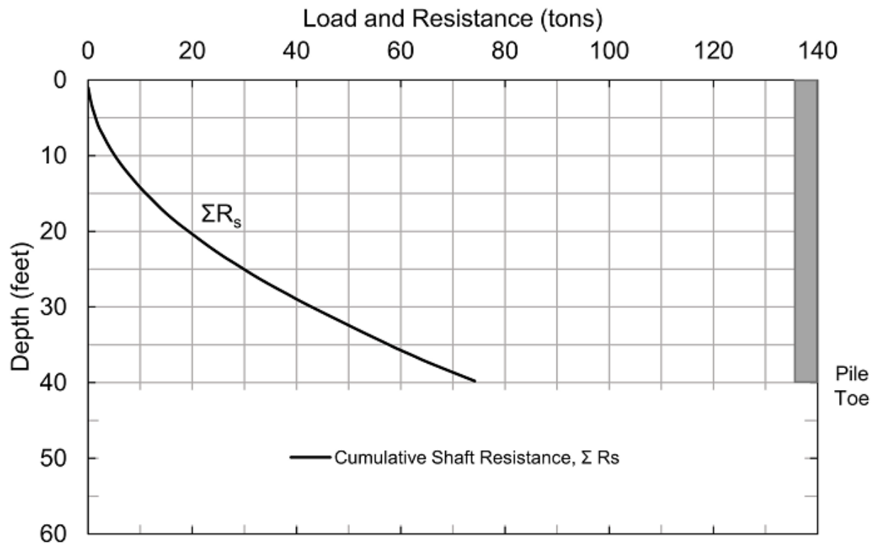
Fig. 5-3. Axial load and resistance plot cumulative shaft resistance vs. depth (after Siegel et al., 2013).
