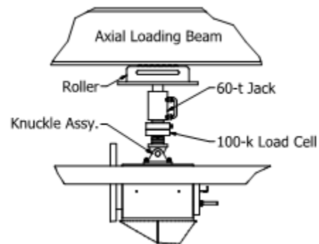
Figure 3.9: Axial Load Setup, \frac{P_d}{A_g f'_c} = 0.05
