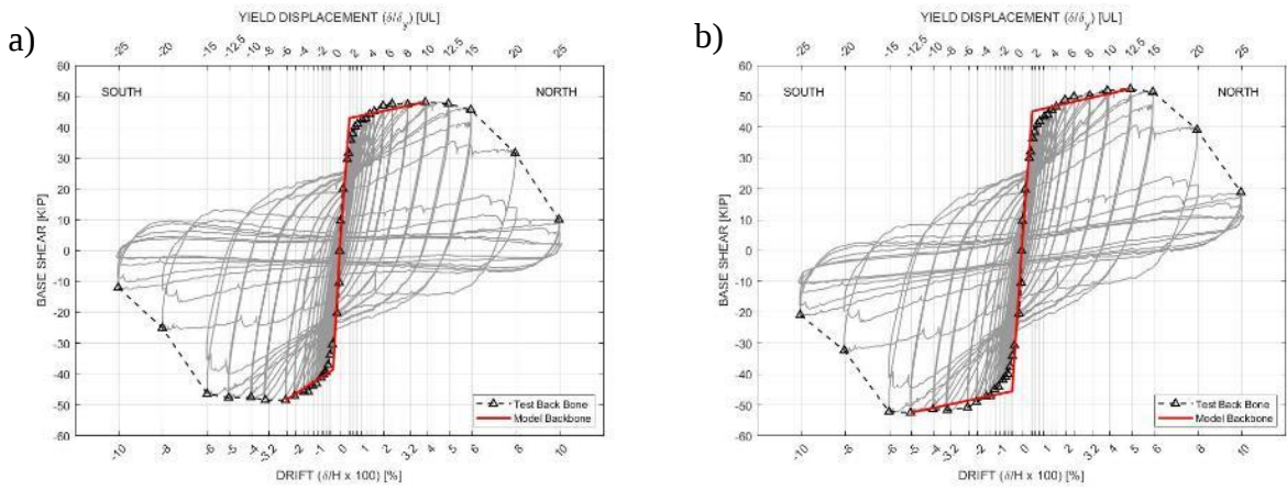
Figure 3.28. Backbone Model Fit for C(CFRP)-4.0-#5(1.4)-0.05: a) Base Shear, b) Effective Base Shear
