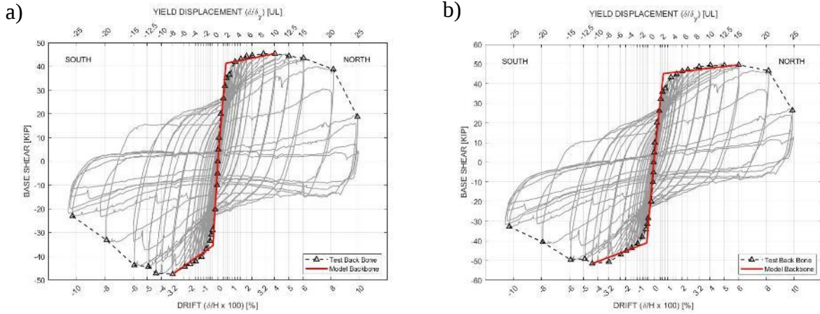
Figure 3.27. Backbone Model Fit for C(CFRP)-4.0-#7(1.3)-0.05: a) Base Shear, b) Effective Base Shear
