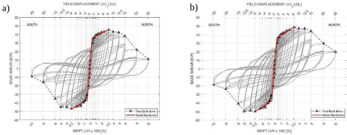
Figure 3.31. Backbone Model Fit for C(CFRP)-4.0-#7(1.3)-0.05-2X: a) Base Shear, b) Effective Base Shear
