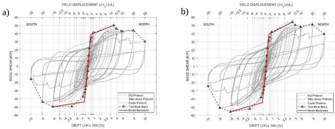
Figure 3.30. Backbone Model Fit for C(CFRP)-4.0-#7(1.3)-0.05-EQ: a) Base Shear, b) Effective Base Shear
