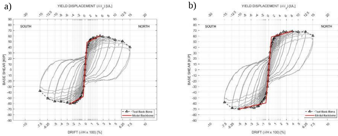
Figure 3.32. Backbone Model Fit for C(CFRP)-4.0-#7(1.3)-0.15: a) Base Shear, b) Effective Base Shear
