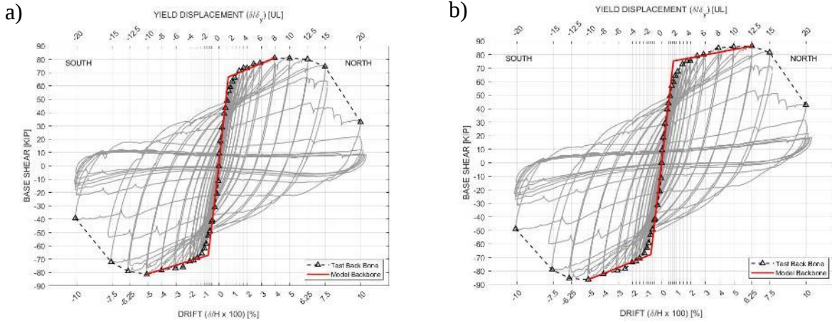
Figure 3.29. Backbone Model Fit for C(CFRP)-4.0-#7(2.7)-0.05: a) Base Shear, b) Effective Base Shear
