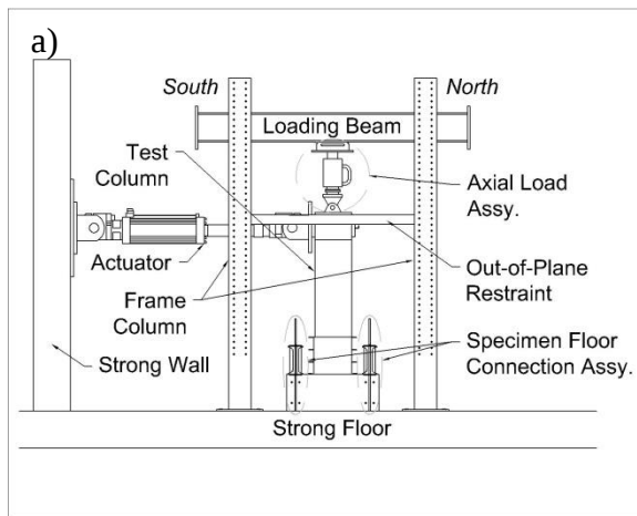
Figure 3.8: Test Set-up, \frac{P_d}{A_g f'_c} = 0.05 : a) Schematic, b) Photo
