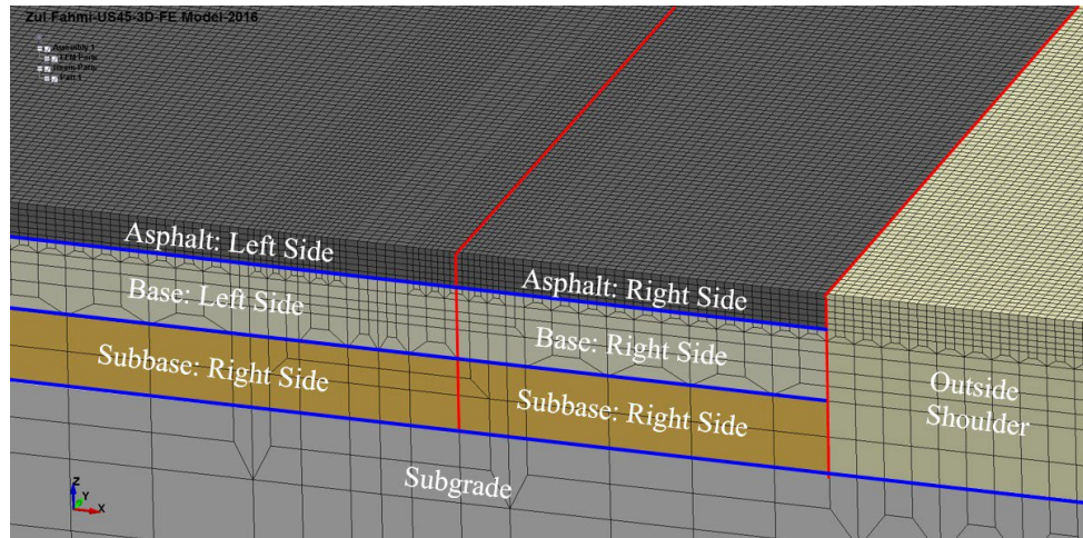
Figure 12. Pavement-subgrade 3D-FE model of uncracked pavement developed
