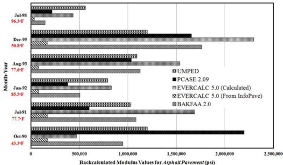
Figure 56. Backcalculated modulus values for asphalt surface layer
