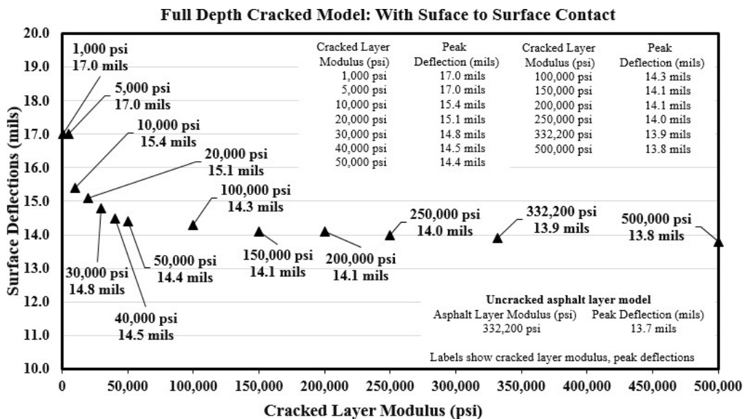
Figure 82. Surface deflections correspond to various cracked layer modulus
