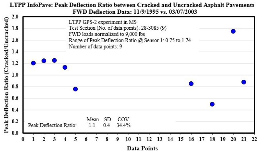
Figure 81. Peak deflection ratios plot of uncracked and cracked pavement for the LTPP test section 28-3085 (deflections normalized to 9,000 lbs.)
