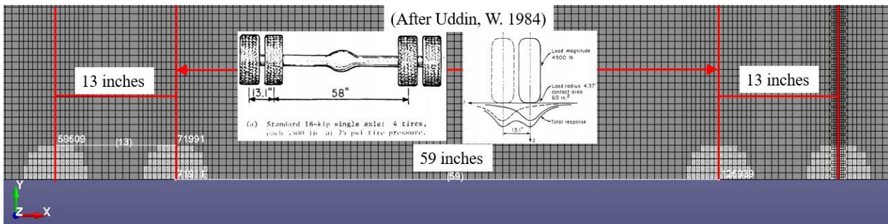
Figure 29. Sketch of an 18-kips single axle truck with 4 tires and contact areas developed in this research
