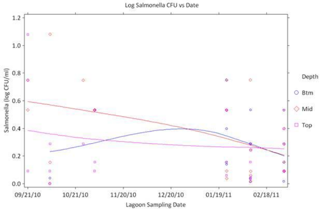
Figure 38 – Concentration of salmonella in manure from the AD lagoon.
