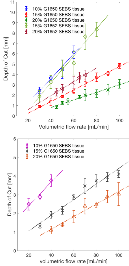
Fig. 16 Experimental DOC of waterjet in SEBS soft tissue simulants vs. volumetric flow rate. (up) DOC vs. Flow Rate for the Needle with 0.32 mm inner diameter (ID) in SEBS Tissue Simulants, and (down) DOC vs. Flow Rate for the Needle with 0.24 mm ID in SEBS Tissue Simulants. The data show the average of 5 tests for each volumetric flow rate, and error bars show the standard deviation of the data.
