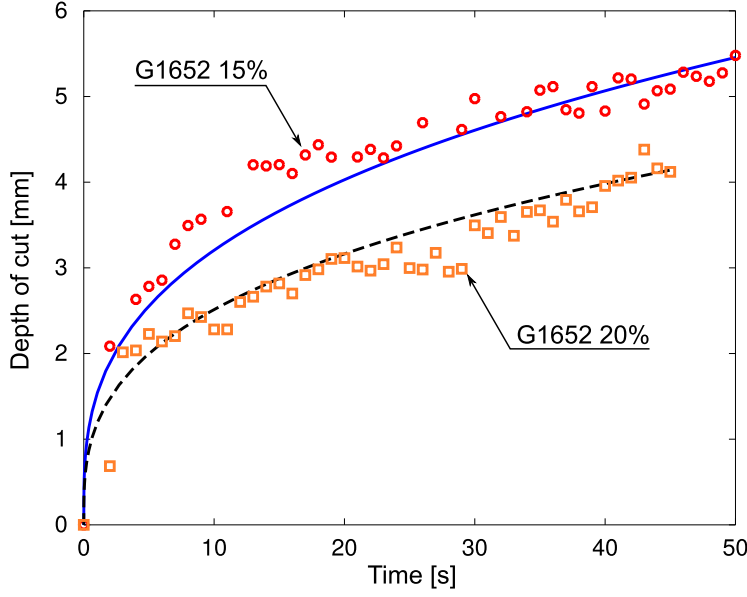
Fig. 19 DOC vs. time for 15% and 20% G1652 tissues; Experimental results (symbols) vs fluid model (lines) with best-fitting \eta . Needle diameter D = 0.32mm , and waterjet velocities (for G1652 15% v = 10.36 \frac{m}{s} , and for G1652 20% v = 14.51 \frac{m}{s} ) are remained constant.
