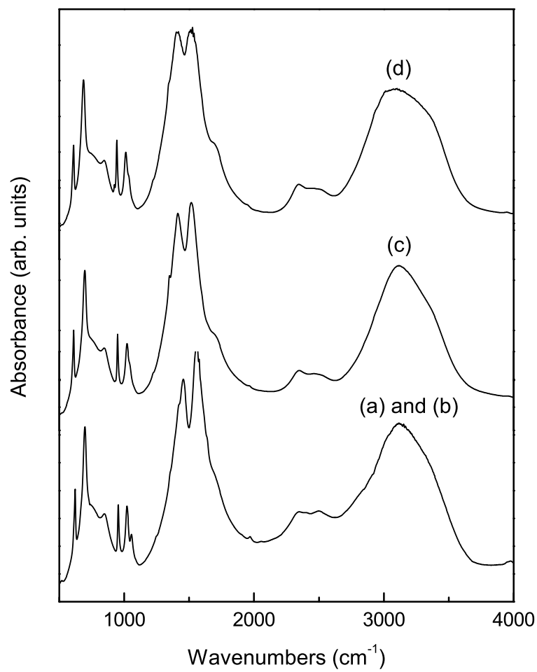
FIG. 4.4. IR absorption spectra of zinc acetate precursors with different ^{13}\text{C} compositions (see Table. 4.1).
