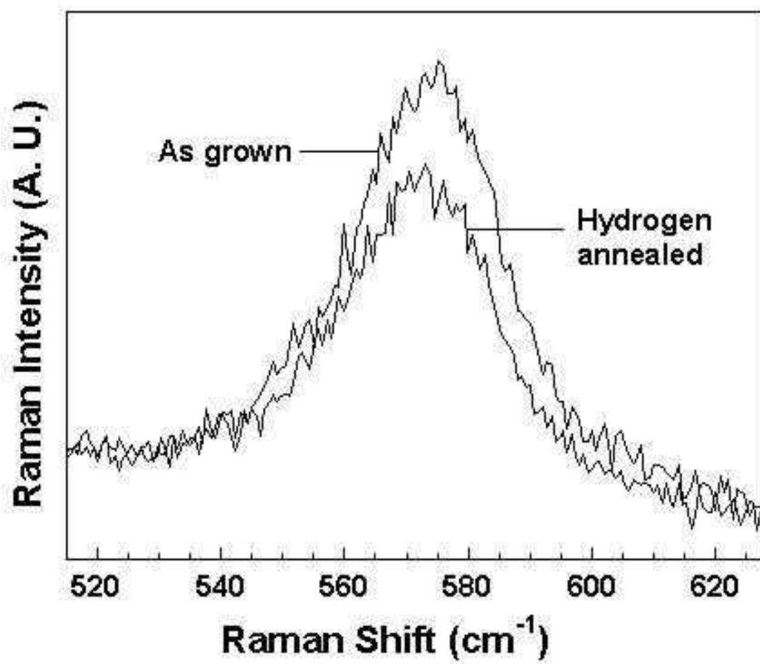
FIG. 5.5. Raman spectra of ZnO nanoparticles.
