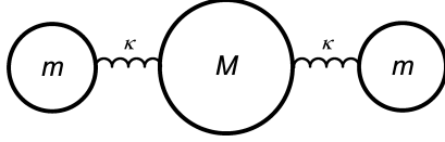
FIG. A.1. Linear tri-atomic molecule.
