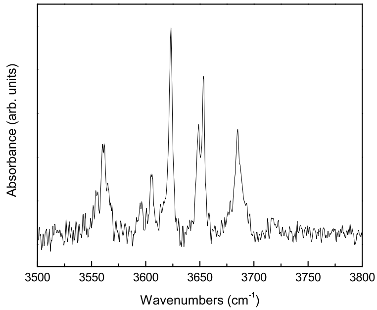
FIG. 6.3. IR absorption spectrum of ZnO:Cu nanoparticles at 9 K (3500-3800 cm⁻¹ region)
