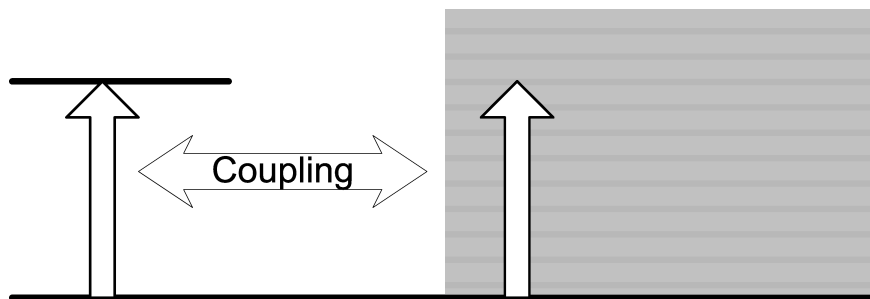
FIG. 7.1. Fano resonance.
