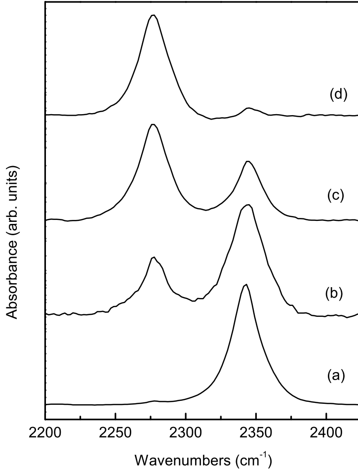
FIG. 4.3. IR absorption spectra of ZnO nanoparticles with different ^{13}\text{C} compositions, (see Table. 4.1).
