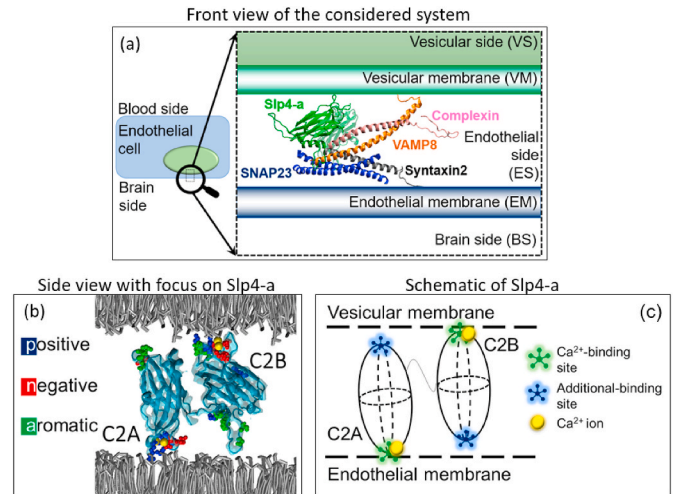
Fig. 2. Structure of the protein system at the pre-fusion stage of a vesicle in BBB. (a) The zoomed-in view of key components: Vesicular membrane, endothelial cell membrane in the brain side, and associate proteins involved in the pre-fusion stage. Protein complex involves in this process includes VAMP8 (orange), Complexin (pink), Syntaxin2 (gray), and SNAP23 (blue), and Slp4-a (green). (b) The new cartoon model for Slp4-a (cyan-colored), which consists of C2A and C2B domains. Each C2 domain shows both the Ca^{2+} binding site and additional binding sites with some important amino acids. Calcium ions (yellow) are shown in the calcium binding site. The additional binding site is located on the opposite side of the Ca^{2+} binding site in each domain. Lipids are shown as gray layers located at the top and bottom sides of the Slp4-a. (c) Sketch of the Slp4-a model with four important regions: two Ca^{2+} binding sites in green and two additional binding regions in blue. (For interpretation of the references to color in this figure legend, the reader is referred to the Web version of this article.)
