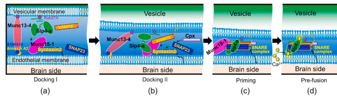
Fig. 1. Schematic of vesicle docking at the pre-fusion stage in BBB exocytosis. (a) Vesicle connects to the endothelial membrane through the first protein bridge (Docking I). Important proteins involved in this bridge are Munc13-4, Rab27A, S100A10, and Annexin A2. (b) The two membranes get closer when Slp4-a binds to Munc18-1 as well as syntaxin2 to form the second docking bridge (Docking II). (c) SNAREs complex formed by the merging of Syntaxin2, VAMP8, and SNAP23 into 4 helix bundle for priming. In this stage, Slp4-a starts to connect with SNAREs and complexin. (d) Calcium ion-dependent pre-fusion, where the protein system could trigger the membrane fusion.
