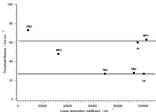
Figure 16. Comparison of the threshold fluences for various polymers as a function of the linear absorption coefficient (Lambert–Beer). PI = polyimide, PEC = poly-ester carbonate, MP = cinnamylidene-malonic ester polymer (for MP1 and MP2 different substituents R are used, see Figure 15), TP = triazene polymer, and TM = the mixed polymer with a triazene and cinnamylidene-malonic ester functionality (see Figure 15). The plot shows, that the polymers with a triazene functional group (TP and TM) reveal much lower threshold fluence values, and that the absorption coefficient has no obvious influence.
