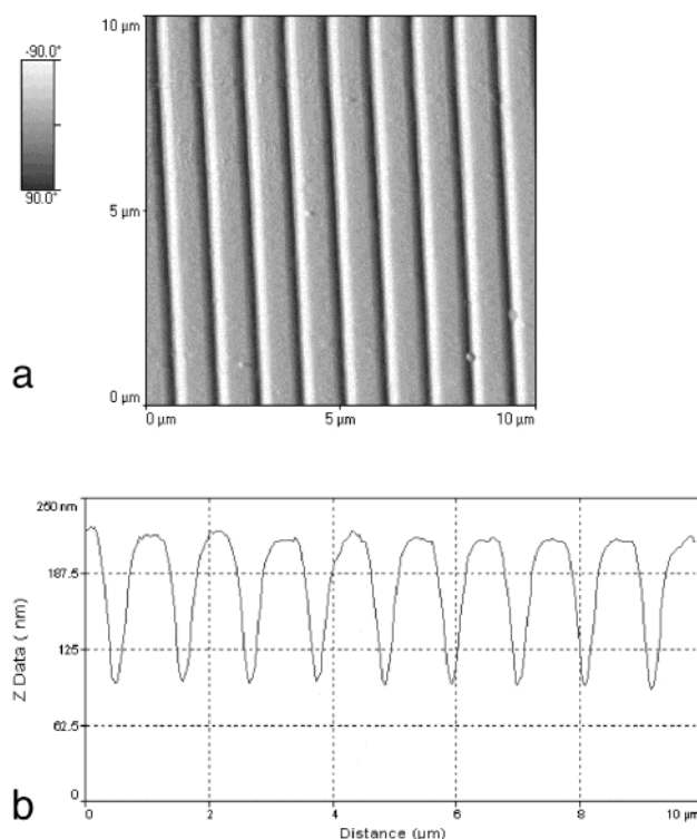
Figure 13. Holographic (interference) grating fabricated into the triazenepolymer with a single pulse of 80 \text{ mJ cm}^{-2} and a 3 ns pulse at 355 nm. The grating has a spacing of 1090 nm, corresponding to the value expected from the experimental setup [Michelson interferometer, where the spacing of the grating ( S ) can be varied by changing the intersection angle ( \theta ) according to S = \lambda/2 \sin^{-1}(\theta/2) ].
