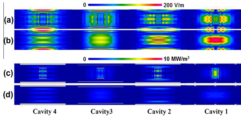
Fig. 3. Electric field distribution (range from 0 to 200 V/m) in the xy plane at the center of the cavity for: (a) loaded cavities, and (b) unloaded cavities. Dissipated power density (range from 0 to 10 MW/m³) in the xy plane at the center of the cavity for: (c) loaded cavities, and (d) unloaded cavities.
