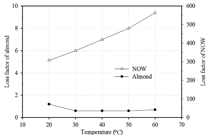
Fig. 1. Comparison of dielectric loss factors ( \epsilon'' ) of almond kernels and navel orangeworm (NOW) larvae as a function of temperature at 27 MHz (updated from Wang et al., 2003b).
