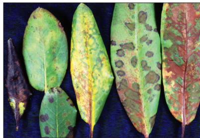
Fig. 19b. Powdery mildew symptoms on upper leaf surfaces as seen on some rhododendron varieties.
