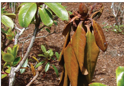
Figure 29a. Wilting and death of branch due to branch canker.
