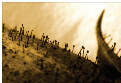
Figure 10a and 10b. Bud blight. Note the tiny black bristles or spores on the bud surface.
