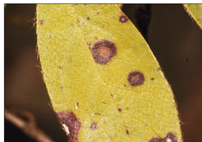
Figure 12c. Leaf spot caused by Septoria spp.
