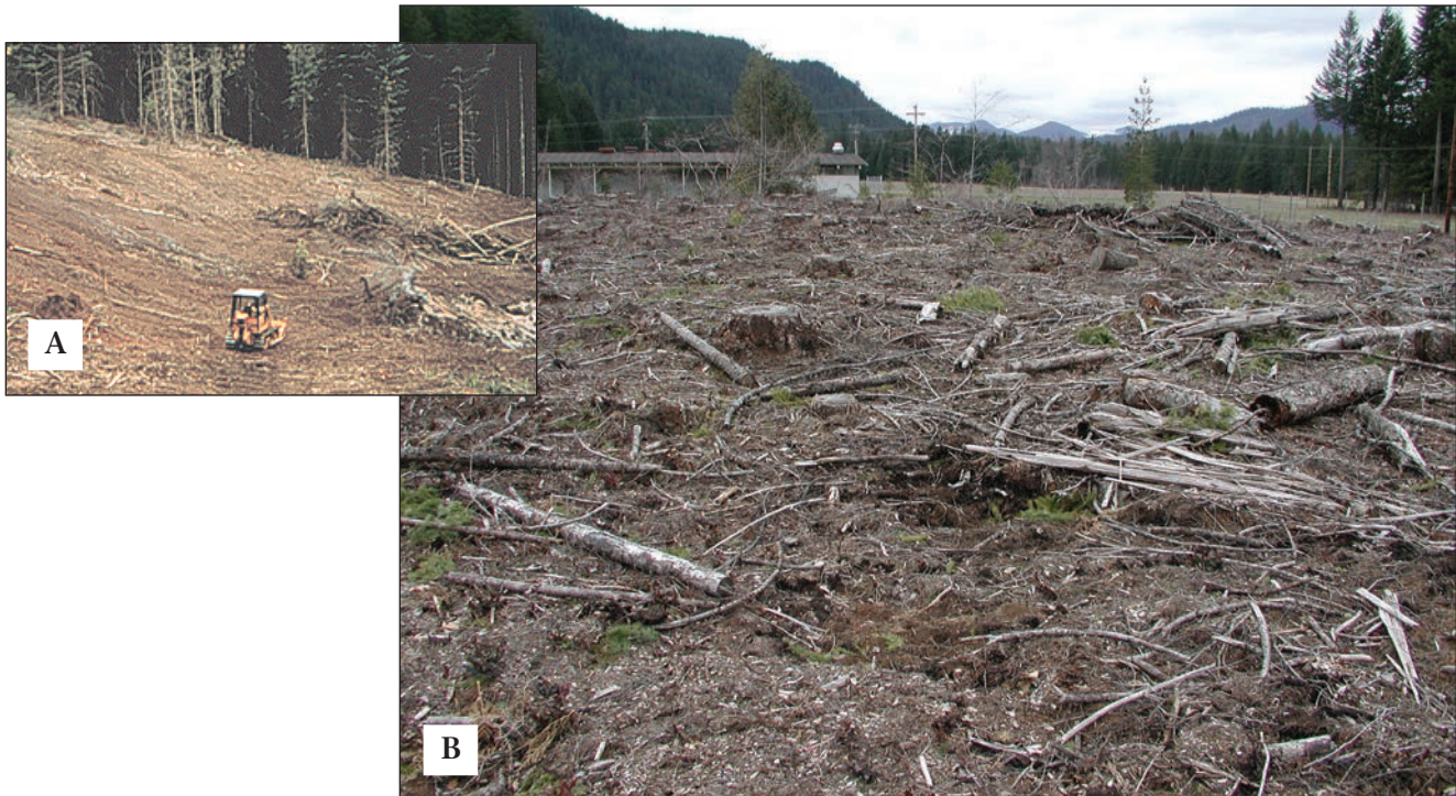
Figure 22. This excessive mechanical site preparation compacts soil, increases its erosion potential, removes organic matter needed for long-term productivity, and costs money for equipment time (A). Good site preparation retains well-distributed slash at amounts compatible with reducing fire risk, controlling competing vegetation, and increasing planting access (B).
