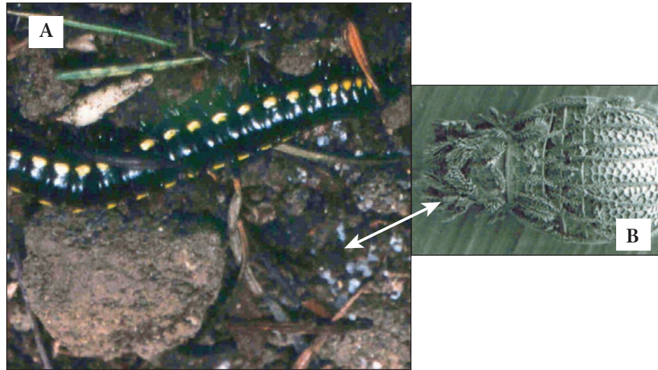
Figure 5. Forest soil biota include an extraordinary array of arthropods, such as this millipede (A) and microscopic turtle mite (B), that are essential for decomposing organic matter and recycling nutrients.
