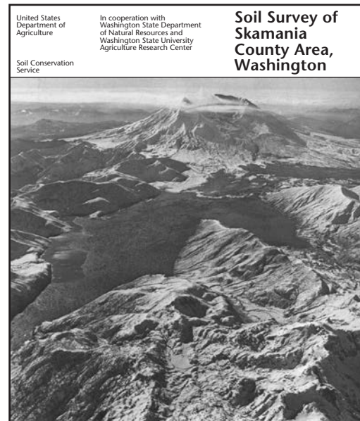
Figure 23. Organized by county, soil surveys provide useful information on forest and wildlife management, agriculture, and construction.
