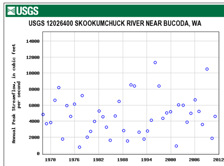
Figure 4. Skookumchuck River Near Bucoda Peak Flows
