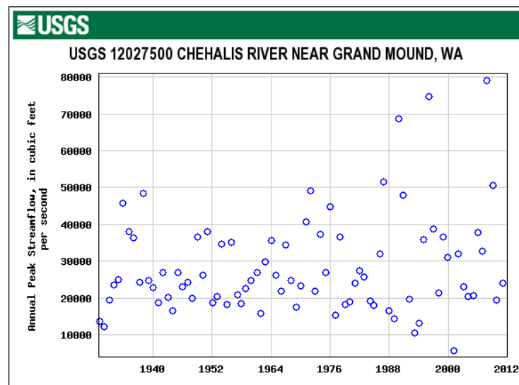
Figure 2. Chehalis River Near Grand Mound Peak Flows
