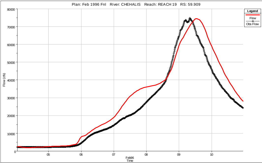
Figure 6. Flow hydrographs for Chehalis River at Grand Mound– February 1996
