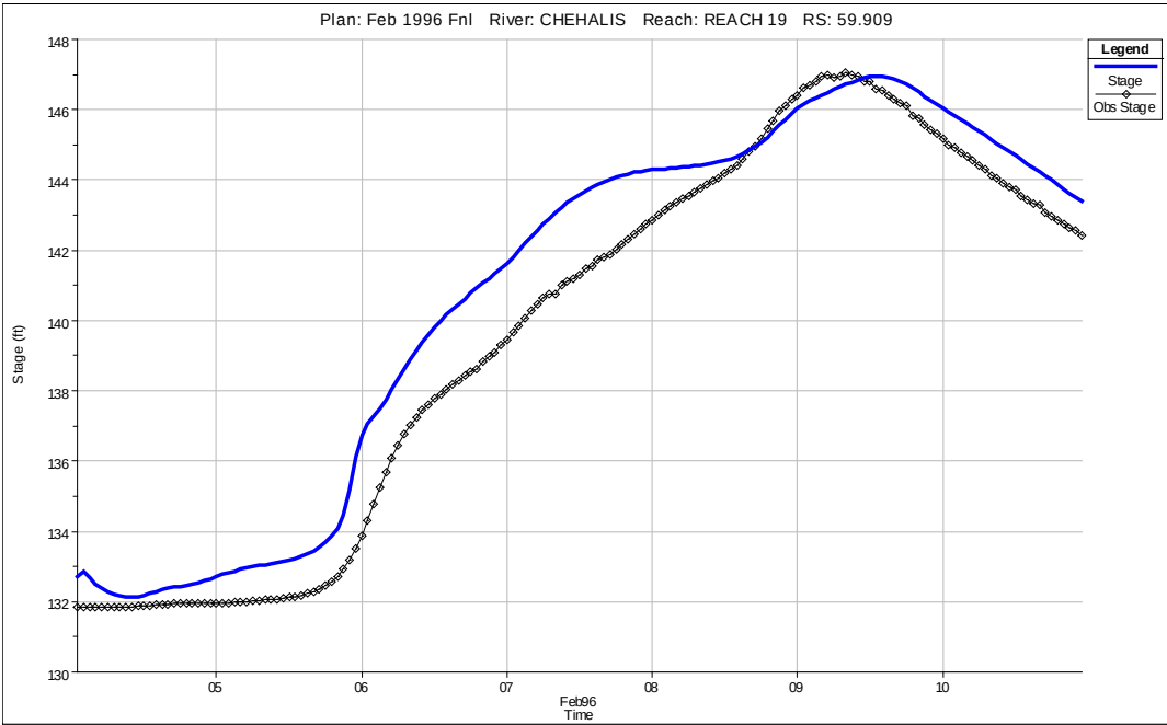
Figure 5. Stage hydrographs for Chehalis River at Grand Mound– February 1996
