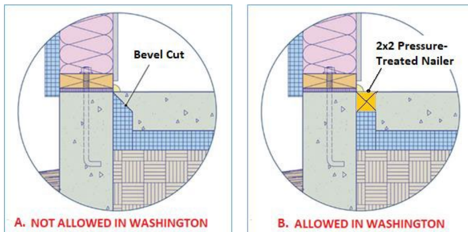
Figure 4 (A) NOT ALLOWED IN WASHINGTON STATE: Illustration of insulation bevel cut in edge insulation allowed under IRC Section N1102.2.10. Chapter 11 has not been adopted in Washington. (B) ALLOWED IN WASHINGTON: Illustration of maximum 2x2 pressure treated nailer at slab edge. Source: Adapted from Holladay, " Fine Homebuilding " to conform with requirements of WSEC-R.
