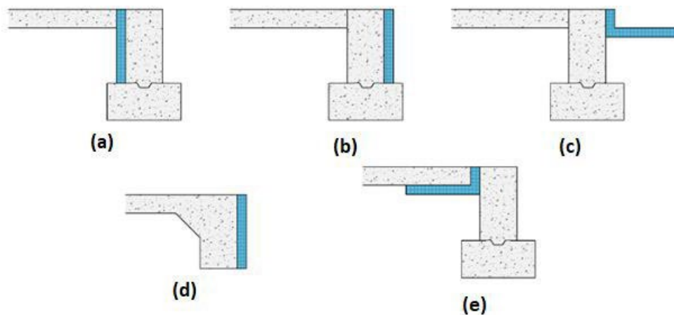
Figure 1 Schematics of acceptable locations for perimeter insulation of unheated on-grade slabs under WSEC-R per Section R402.2.9. (Not all details are shown in these schematics). Adapted from Overbey to conform with 2018 WSEC-R1. 1
