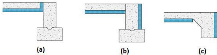
Figure 2 Schematics of acceptable locations for perimeter insulation of heated on-grade slabs under WSEC-R per Section R402.2.9. (Not all details are shown in these schematics).
