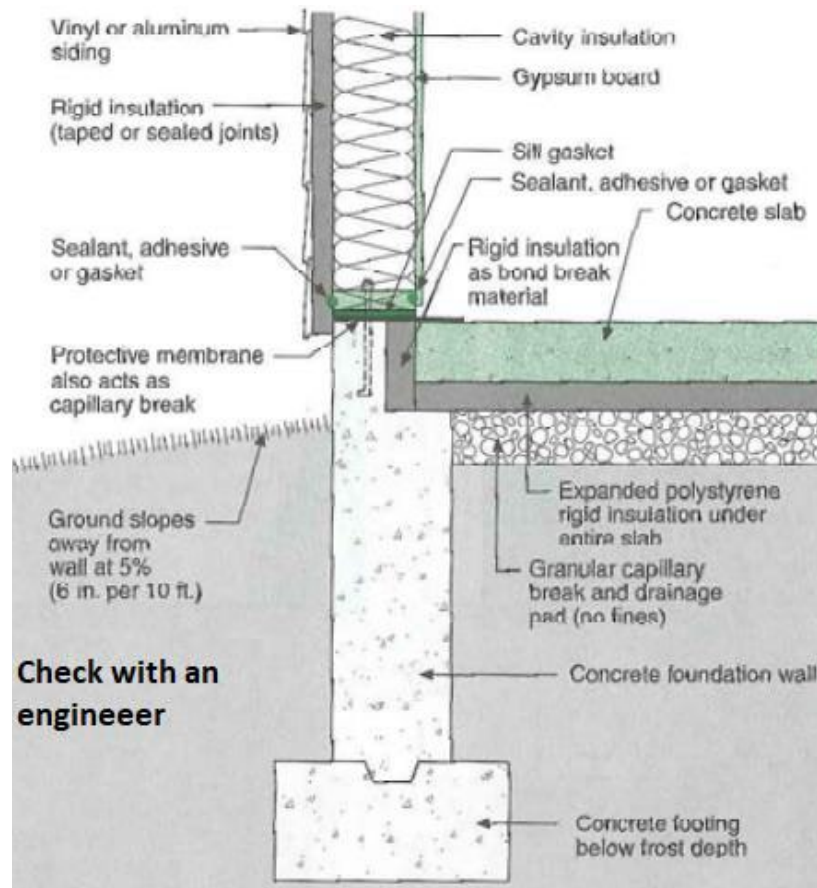
Figure 7 Strategy to avoid a bevel cut in perimeter insulation: cantilever the sill plate of the above-grade wall out over the top edge of the insulation. Source: Turns, PHRC
