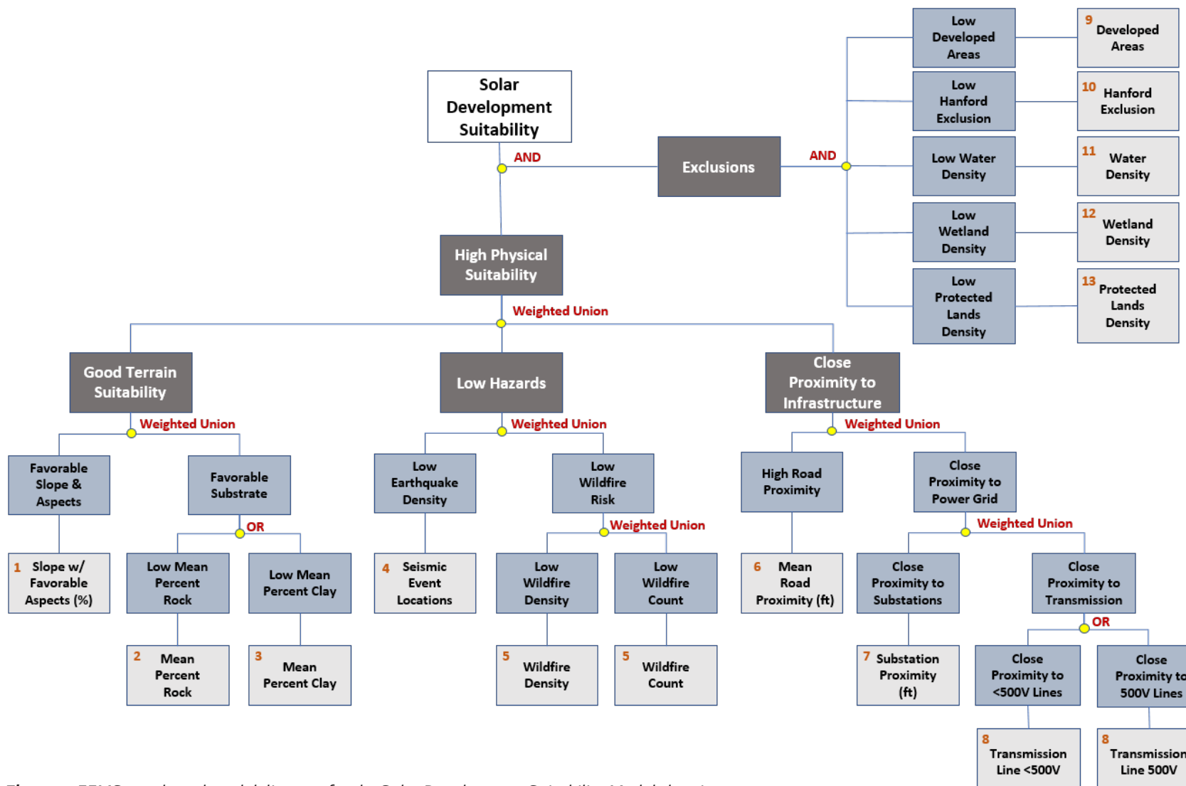
Figure 5. EEMS tree-based model diagram for the Solar Development Suitability Model showing individual model inputs (gray boxes), intermediate map after fuzzy command (blue boxes), high-level nodes (dark gray boxes with white text), and apex map (white box at the top of the diagram). Logic operators are indicated in dark red text (see Appendix B for operator descriptions). Orange numbers in the gray boxes correspond to the data sources in Table C-1 in Appendix C .
