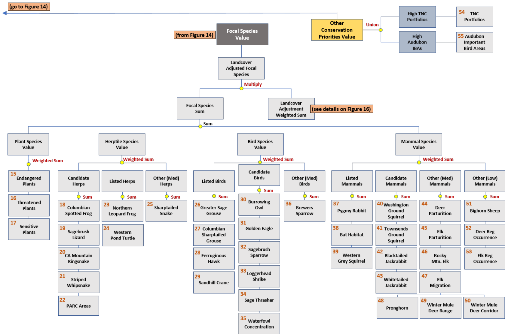
Figure 15. EEMS tree-based model diagram for the Conservation Value Model showing individual model inputs (gray boxes), intermediate map after fuzzy command (blue boxes), high-level nodes (dark gray boxes with white text), and apex map (white box at the top of the diagram). The yellow box depicts a node that denotes support without impacting final map results. Logic operators are indicated in dark red text (see Appendix B for descriptions). Orange numbers in the gray boxes correspond to the data sources in Table C-4 in Appendix C .
