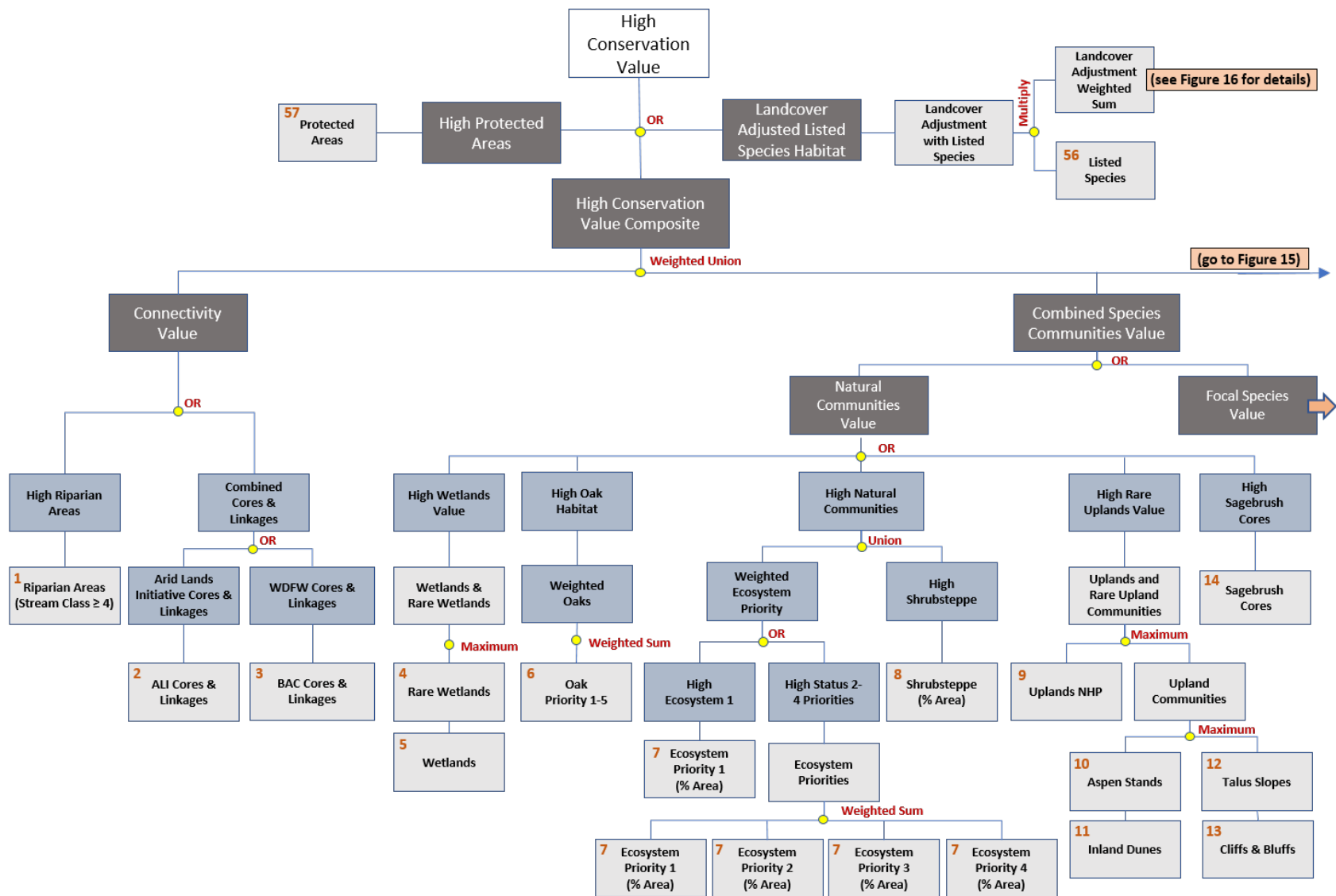
Figure 14. EEMS tree-based model diagram for the Conservation Value Model showing individual model inputs (gray boxes), intermediate map after fuzzy command (blue boxes), high-level nodes (dark gray boxes with white text), and apex map (white box at the top of the diagram). Logic operators are indicated in dark red text (see Appendix B for descriptions). Orange numbers in the gray boxes correspond to the data sources in Table C-4 in Appendix C .
