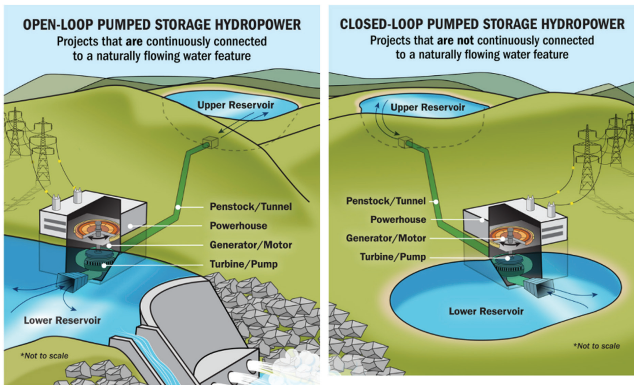
Figure 2. Open-Loop and Closed-Loop Pumped Storage Hydropower
