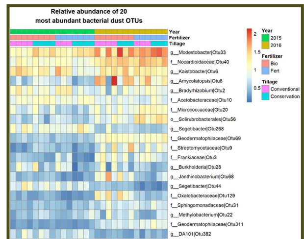
Figure 1. Heatmap of the relative abundances ( \text{Log}_2(1+X) -transformed sequence counts) of the 20 most abundant bacterial OTUs.
